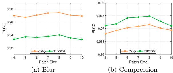
Fig. 8: Impact of image patch size on performance.
